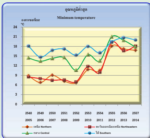
Figure 70 Annual temperature by region, 2005-2014
