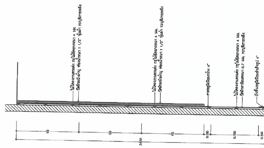
SECTION - C SCALE 1:20
